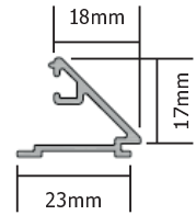
AW513 28mm Bevel Bead
