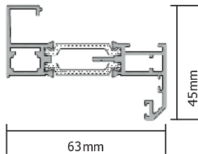
AW690 SL Bevel Sash
