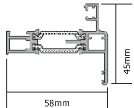
AW686 SL Stepped Sash
