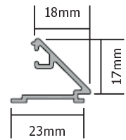
AW513 28mm Bevel Bead
