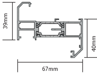
AW611 Euro Bevel Sash
