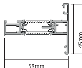
AW685 SL Flat Sash
