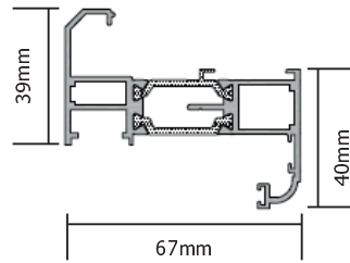
AW613 Euro Ogee Sash
