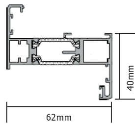
AW624 Flat Sash
