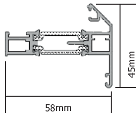
AW614 SL Bevel Sash
