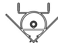
Cornerpost Ali
