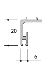
P-00-211 Threshold Adaptor
