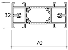
P-06-300 Floating Mullion
