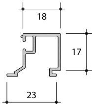
AW660 28mm Square Bead
