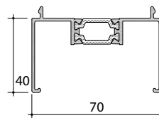
AW728 40mm Add-on
