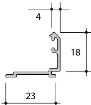
AW666 40mm Bead
