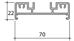
P-06-131 22mm Low Threshold
