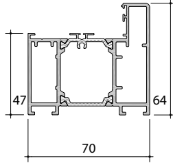
P-06-202 Square Sash
