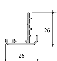
P-00-210 Rebate Adaptor
