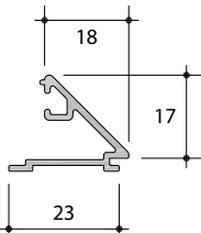
AW513 28mm Flat\ Bevel Bead
