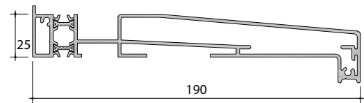
AW544 190mm Cill
