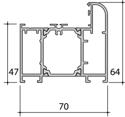
P-06-200 Softline/ Round Sash
