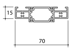
P-06-301 Slave Adaptor
