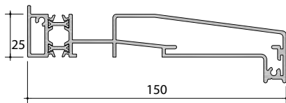
AW542 150mm Cill
