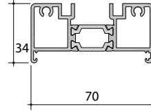
P-06-130 34mm Low Threshold
