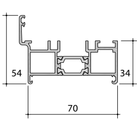
P-06-100 Frame
