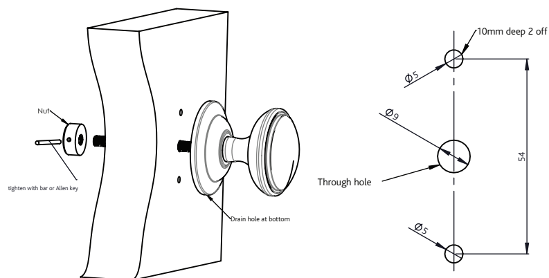
Through Fix
