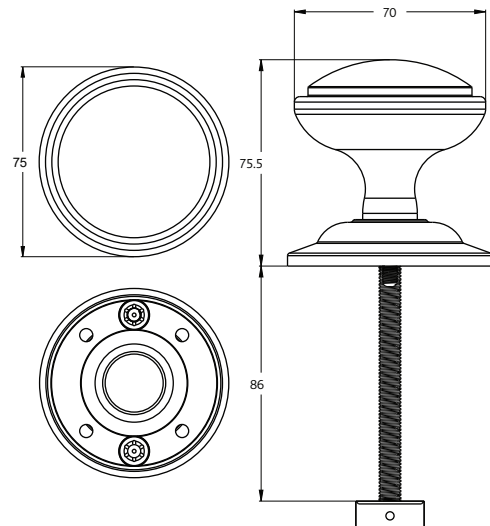
Face Fix
