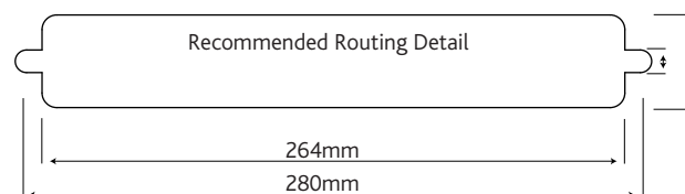
Panel Sleeve Set 20mm-40mm
