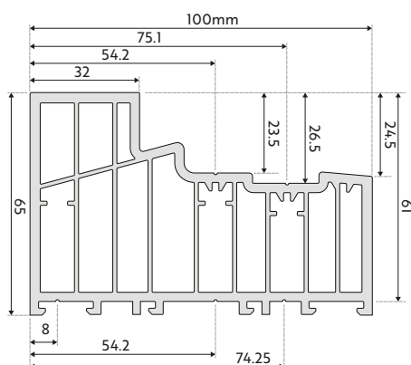
R 2 FRAME
