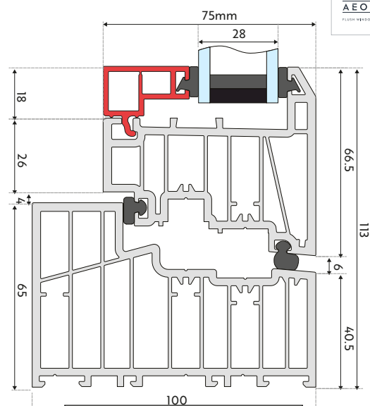
R9 FRAME FLUSH SASH & DECORATIVE BEAD
