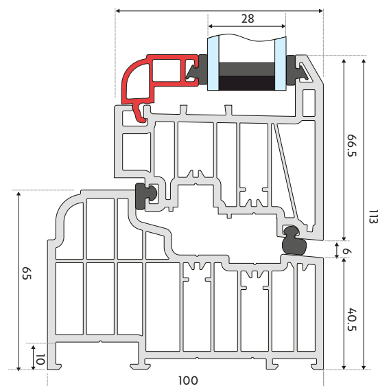
R 2 FRAME FLUSH SASH & SQUARE BEAD
