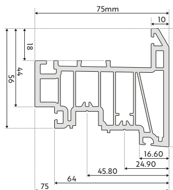
R7 SASH
