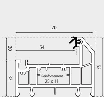
SLIM OUTERFRAME 52mm (5 CHAMBER)
