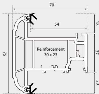
'T' SASH 75mm (5 CHAMBER)
