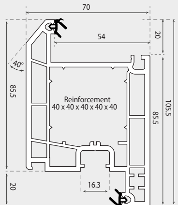
DOOR 'Z' SASH 105.5mm
