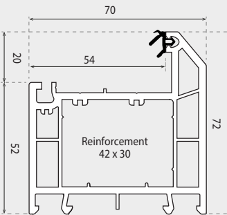
LARGE OUTERFRAME 72mm (3 CHAMBER)
