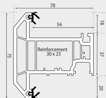
CASEMENT 'T' SASH 75mm (5 CHAMBER)
