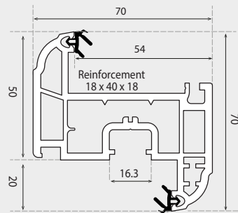
TILT/TURN SASH 70mm
