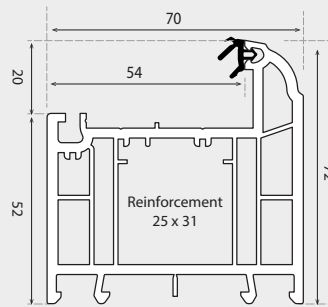
UNIVERSAL OUTERFRAME 72mm (5 CHAMBERS)
