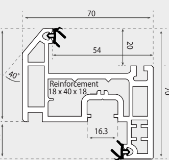
TILT/TURN SASH 70mm
