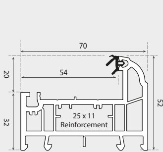
SLIM OUTERFRAME 52mm (5 CHAMBERS)
