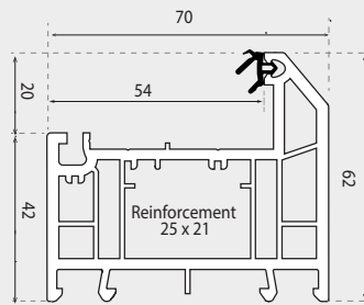
INTERMEDIATE OUTERFRAME 62mm (5 CHAMBER)
