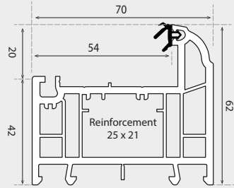
INTERMEDIATE OUTERFRAME 62mm (5 CHAMBERS)
