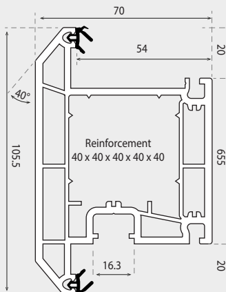
DOOR 'T' SASH 105.5mm
