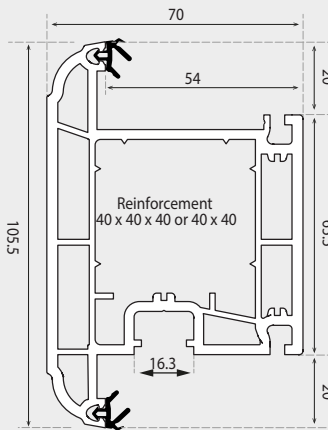
DOOR 'T' SASH 105.5mm
