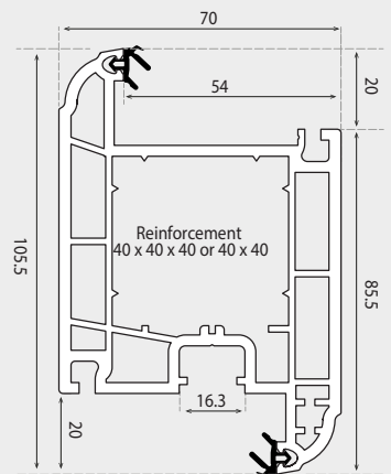
DOOR 'Z' SASH 105.5mm
